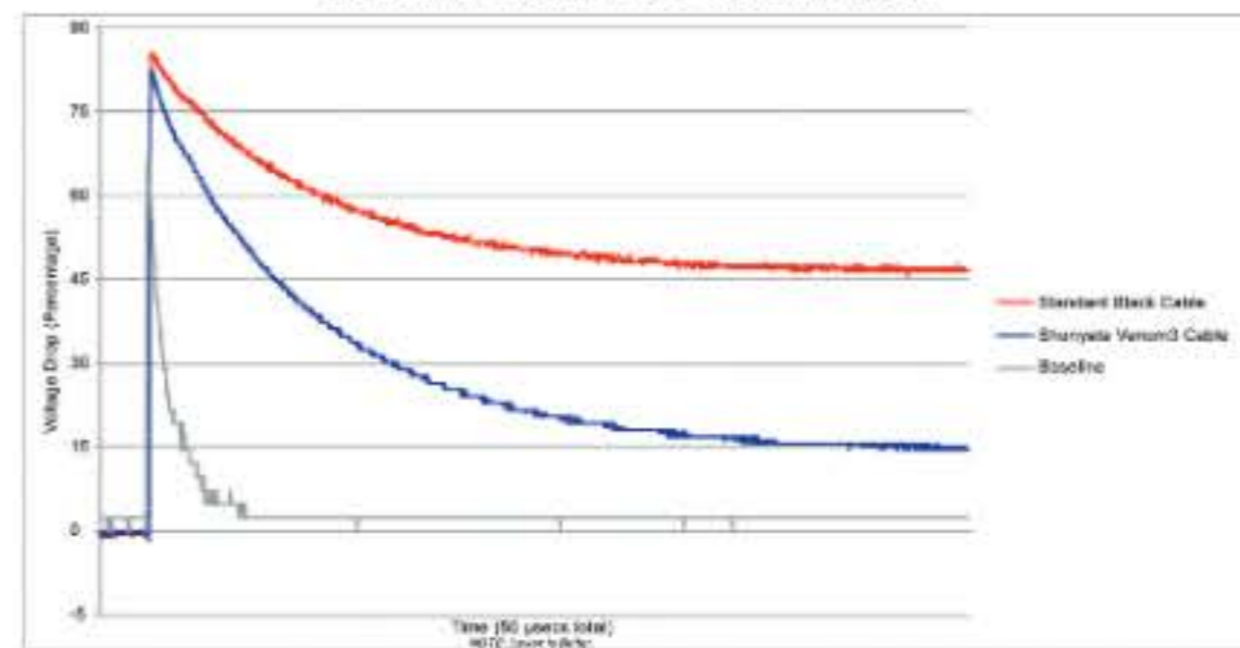
DTCD VOLTAGE DROP COMPARISON
