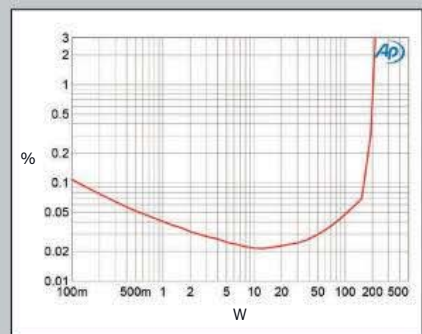
Fig.12 Simaudio Moon Neo 340i, THD+N (%) vs 1kHz continuous output power into 4 ohms.
