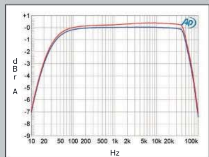
Fig.6 Simaudio Moon Neo 340i, phono input, response with RIAA correction (left channel blue, right red) (1dB/vertical div.).
