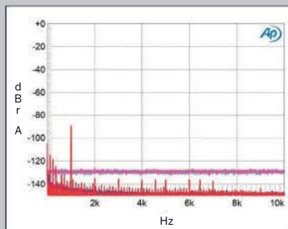
Fig.3 Simaudio Moon Neo 340i, S/PDIF input, 44.1kHz data, spectrum with noise and spurious of dithered 1kHz tone at -90dBFS with 16-bit data (left channel cyan, right magenta), 24-bit data (left blue, right red) (20dB/vertical div.).
