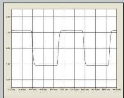
Fig.9 Simaudio Moon Neo 340i, small-signal, 10kHz squarewave into 8 ohms.
