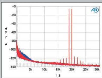
Fig.7 Simaudio Moon Neo 340i, phono input, HF intermodulation spectrum, DC-30kHz, 19+20kHz at 1V peak into 100k ohms (linear frequency scale).
