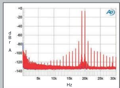
Fig.16 Simaudio Moon Neo 340i, HF intermodulation spectrum, DC-30kHz, 19+20kHz at 100W peak into 4 ohms (linear frequency scale).
