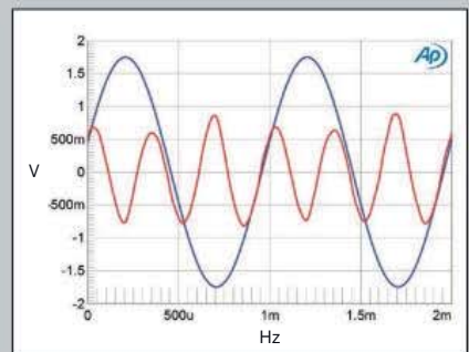
Fig.14 Simaudio Moon Neo 340i, 1kHz waveform at 50W into 8 ohms, 0.042% THD+N (blue); distortion and noise waveform with fundamental notched out (red, not to scale).
