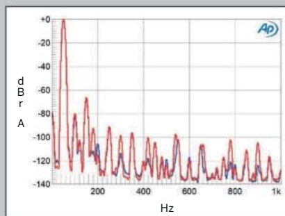
Fig.15 Simaudio Moon Neo 340i, spectrum of 50Hz sine wave, DC-1kHz, at 100W into 4 ohms (linear frequency scale).
